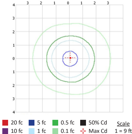
Footcandle Plot for 15W 4' T8 Tube @ 9 ft
