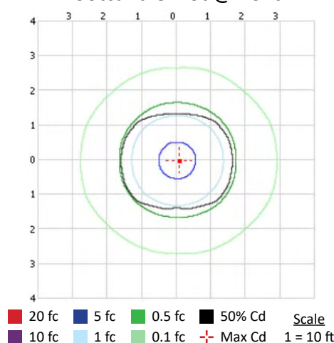
Footcandle Plot @ 10 ft
