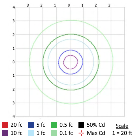
Footcandle Plot @ 20 ft
