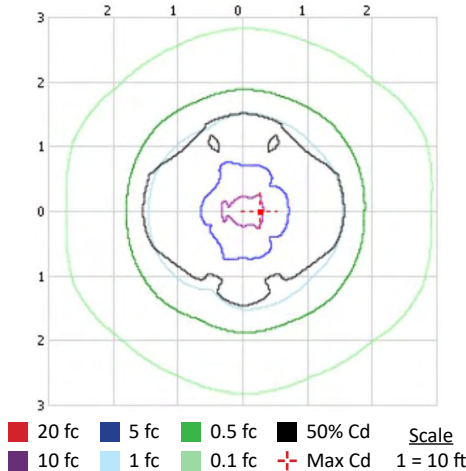
Footcandle Plot @ 10 ft
