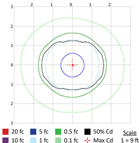
Footcandle Spread @ 9 ft
