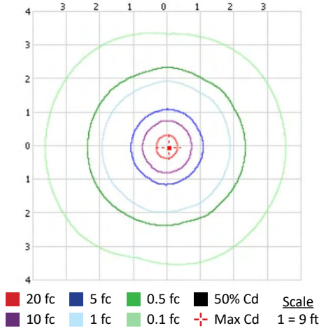
Footcandle Plot for 18W 4' T8 Tube @ 9 ft
