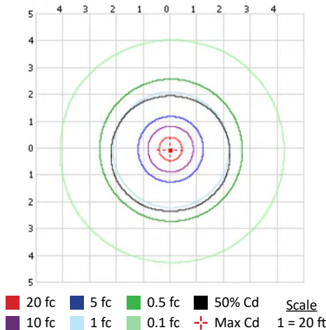
Footcandle Plot @ 20 ft
