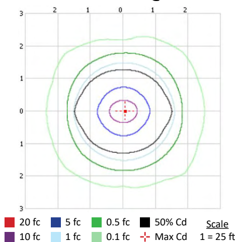
Footcandle Plot @ 25 ft
