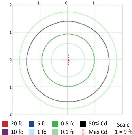
Footcandle Plot @ 9 ft
