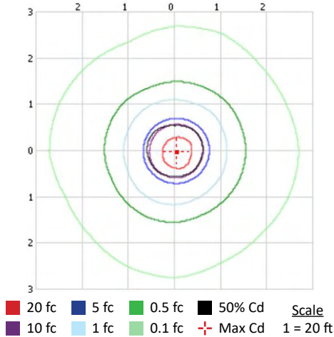
Footcandle Plot for 200W High Bay @ 20 ft
